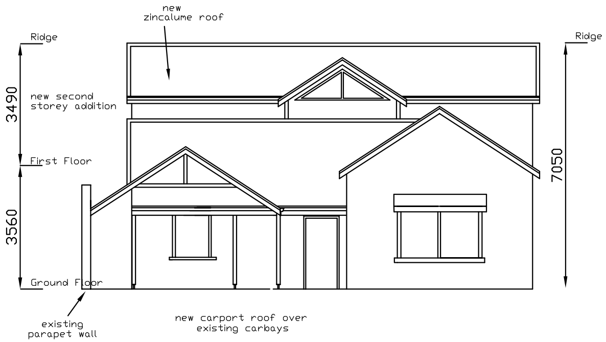
SOUTH ELEVATION
